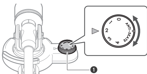
1 Anti-Skating-Drehrad
